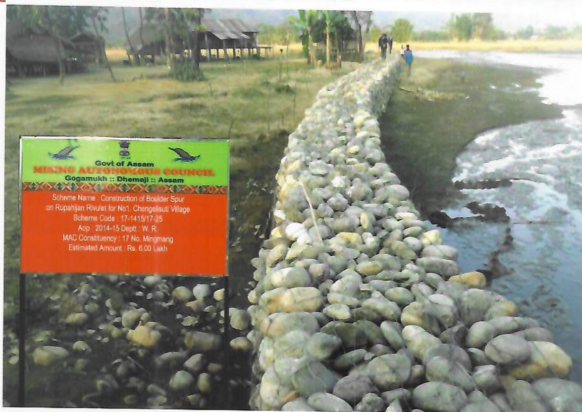
Construction of Boulder Spur on Rupahijan to Protect Sengelisuti Village in Mingmang Constituency
